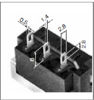
Solder Lug(ON-ON)
