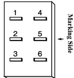
Terminal Diagram
