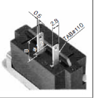
Quick Connect terminal#110 (ON-OFF)
