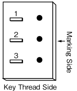
Terminal Diagram
