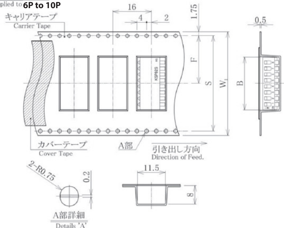
The Dimension of each part (mm)
