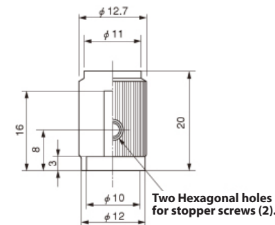
For the assembly of aluminum Knurring, please use a hexagonal wrenth #6-32UNC.
