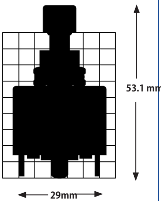
Silhouette (APD21)
