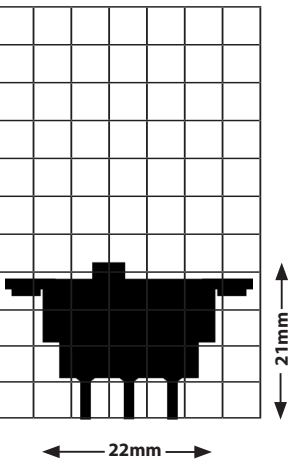
Silhouette (CSD01)
