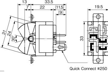
Quick Connect #250
