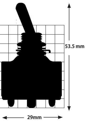
Silhouette (ATA21)
