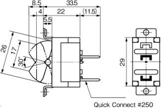
Quick Connect #250
