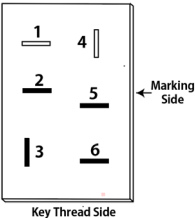
Terminal Diagram
