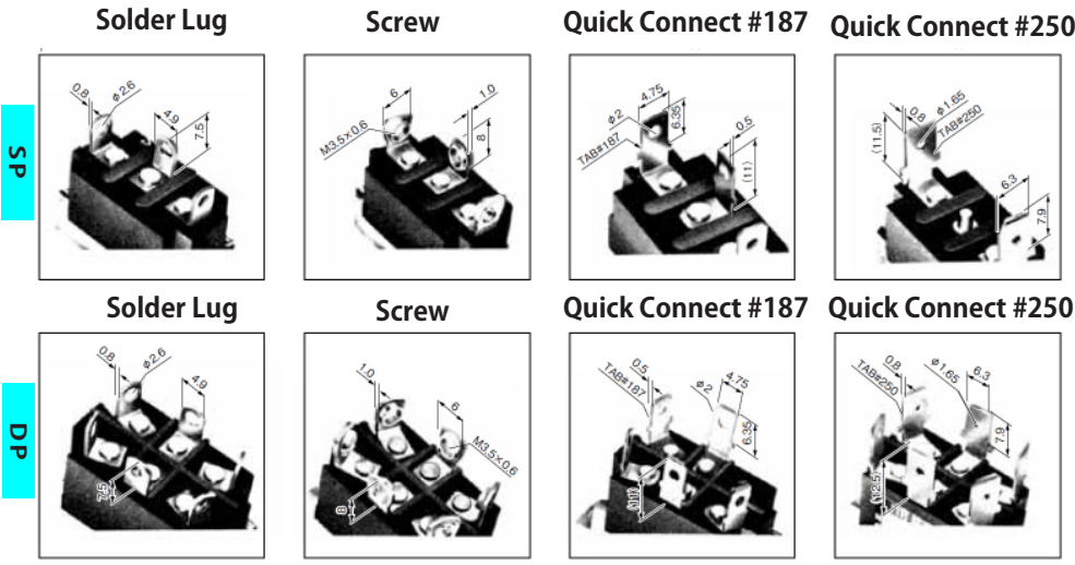
Silhouette (ATA21)
