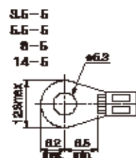
Applicable cramping terminals
