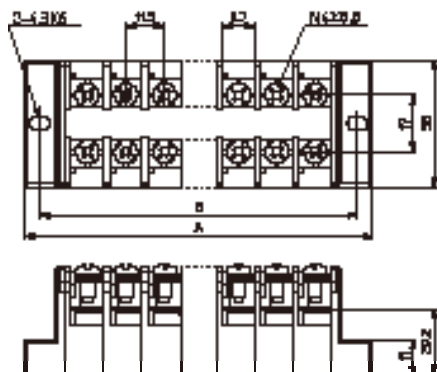
Appearance diagram (Unit:mm)
