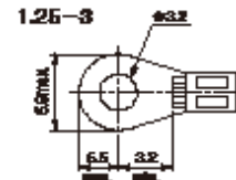
Applicable crimping terminals
