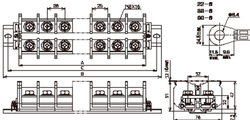
Appearance diagram (Unit:mm)
