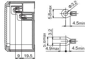
Applicable Cramping Terminal
