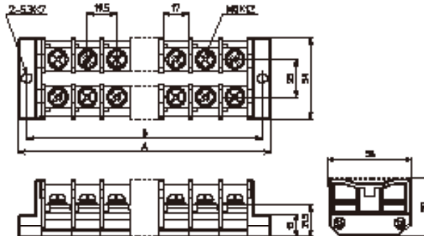
Appearance diagram (Unit:mm)
