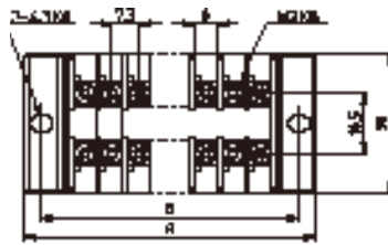
Appearance diagram (Unit:mm)
