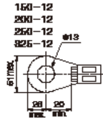
Applicable cramping terminals
