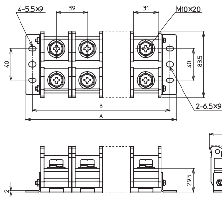
Appearance diagram (Unit:mm)
