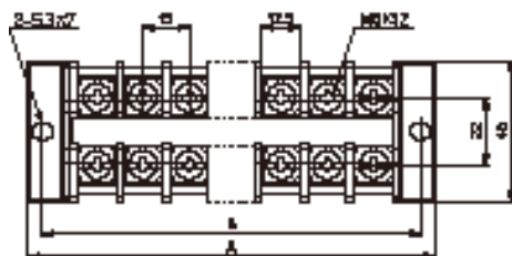
Appearance diagram (Unit:mm)
