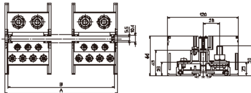
Appearance diagram (Unit:mm)
