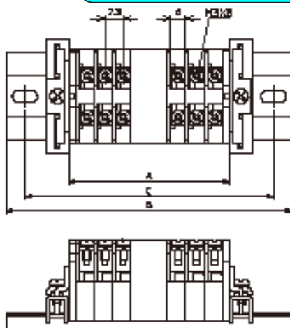
Appearance diagram (Unit:mm)
