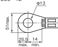
Applicable crimping terminals
