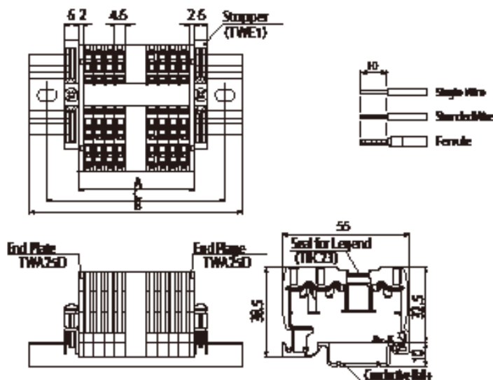
Appearance diagram (Unit:mm)
