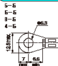
Applicable crimping terminals
