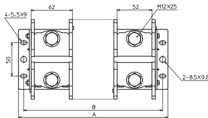
Appearance diagram (Unit:mm)
