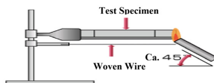
Horizontal Test Method
