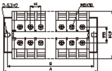
Appearance diagram (Unit:mm)
