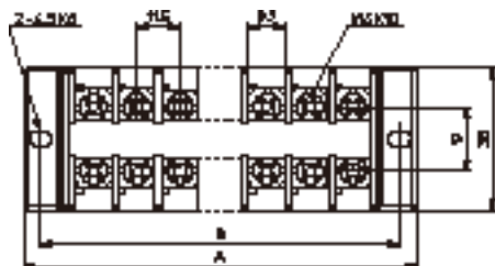
Appearance diagram (Unit:mm)
