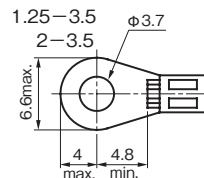
Applicable crimping terminals
