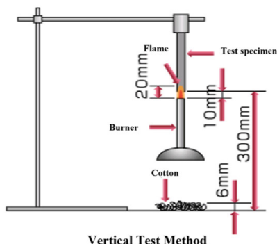
Vertical Test Method
