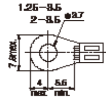
Applicable cramping terminals
